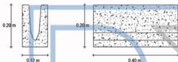
Block hueco Dala "U" 12-20-40
